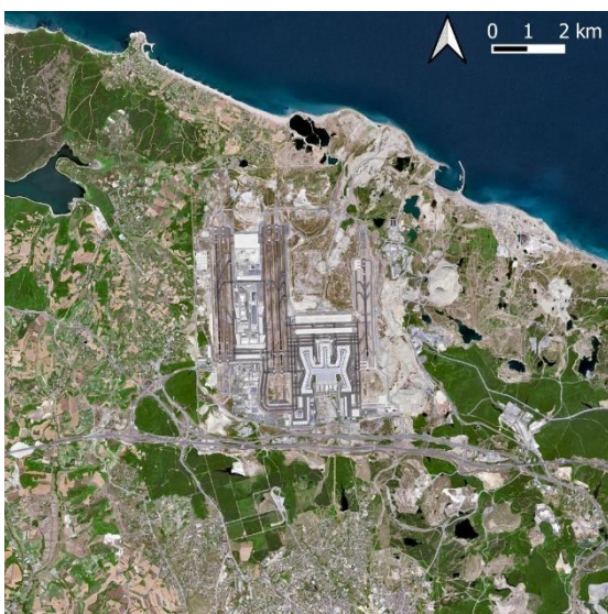
Sentinel-2, 2023-07-23
